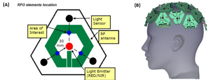
Sensor design (A) and assembly (B)
